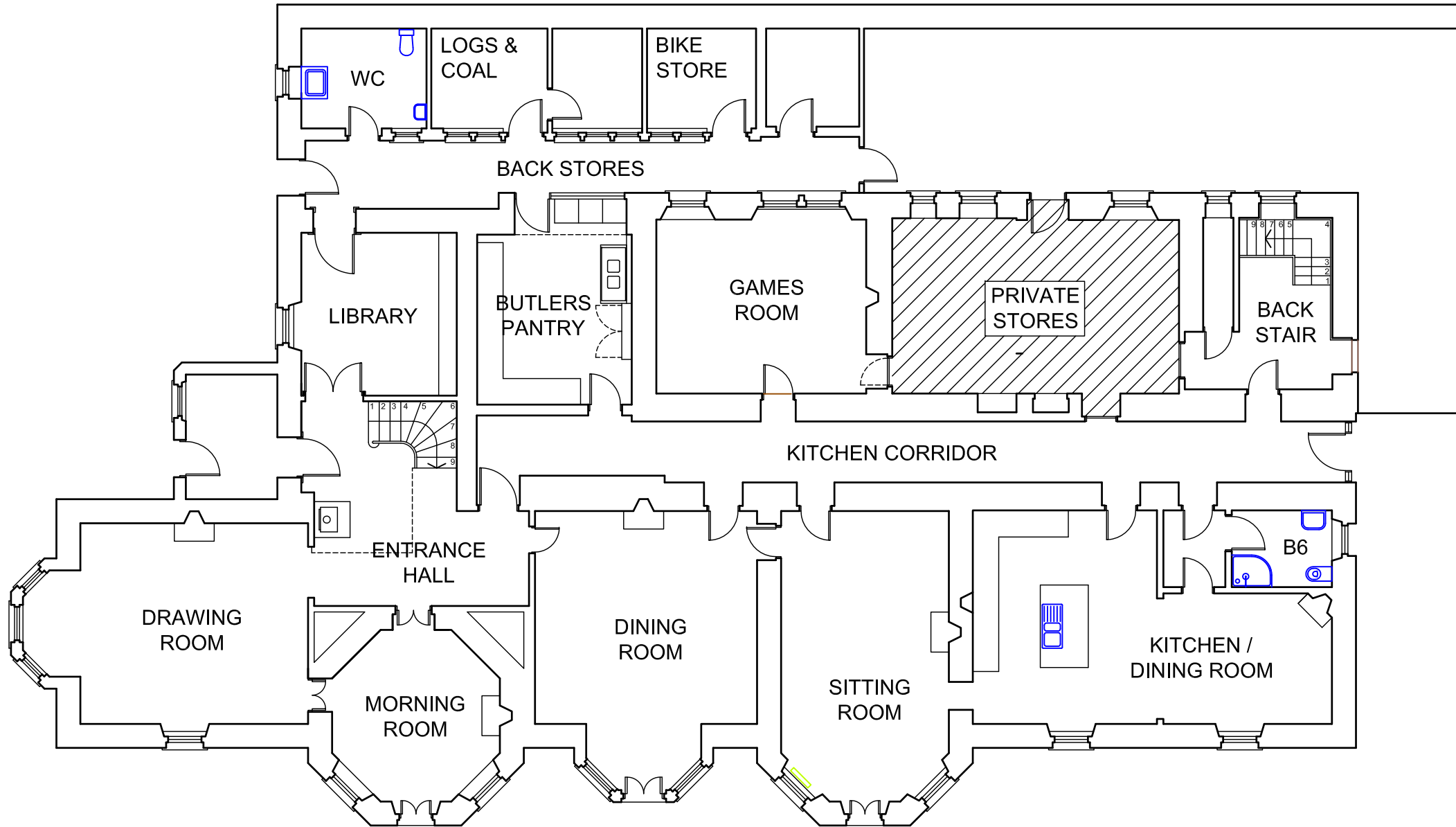
EASTWOOD HOUSE Ground Floor Plan
